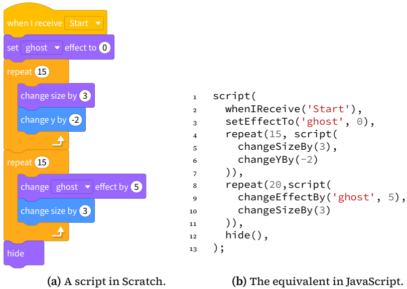
Listing 5.4. An example of how a Scratch program can be represented using the abstractions provided by Itch.
