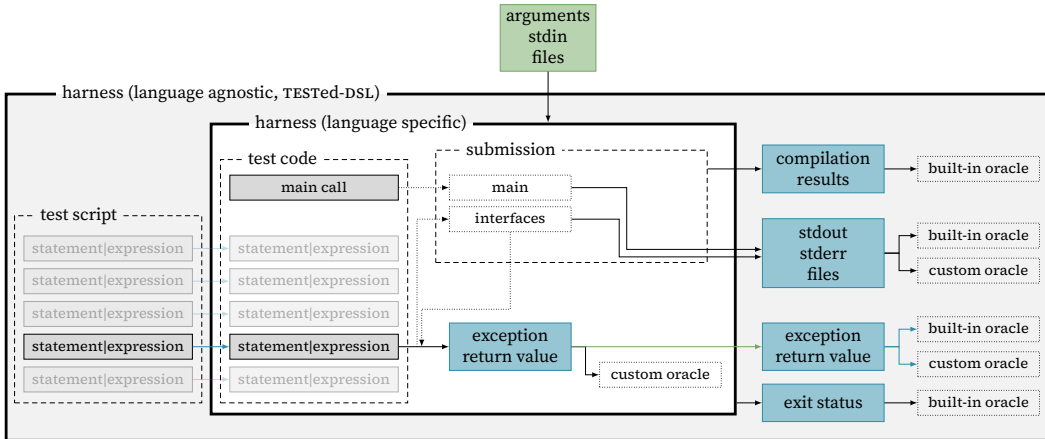
Figure 3.3. Architecture of the test execution engine of TESTED. Since TESTED supports both input/output testing and unit testing, its architecture is a combination of figures 3.1 and 3.2. TESTED achieves this by running a language-specific harness (white box) within the language-agnostic test harness (grey box). Assessing a submission for a single test case again comes down to compiling the submission along with test code into an executable test harness. The input data are passed to the executable, and the test script consists of a set of statements and expressions. However, the strongly typed values, expressions and statements in the test script may now be in a language-agnostic representation. Before compilation, the test script is transformed (blue arrows) into language-specific test code. While the main call interacts with the main function of the submission, other tests access public interfaces of the submission (a single statement/expression is illustrated here). If a language-specific oracle is used, it is included in the language-specific harness. Otherwise, the strongly-typed outputs , together with the outputs from the main function, are processed in the language-agnostic harness. To make this possible, strongly-typed outputs are transformed from a language-specific representation into a language-agnostic representation (green arrow). Finally, oracles in the language-agnostic harness evaluate the outputs. To make this possible, strongly typed values are converted in to the language-specific representation of the oracle (blue arrow).
