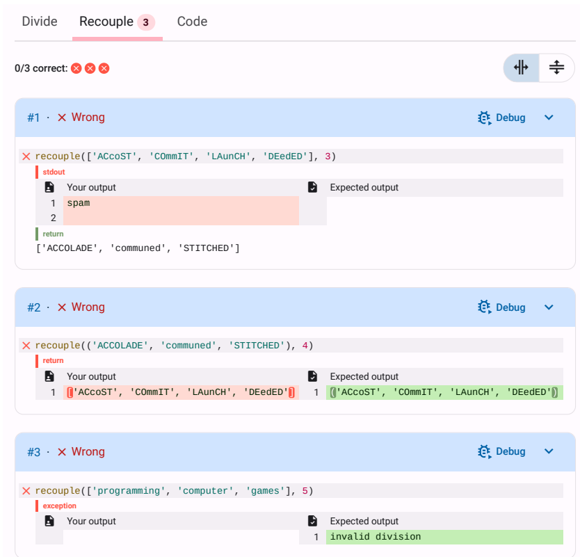
Figure 3.5. Dodona rendering of test results after TESTed validated a wrong Python submission for a programming exercise configured with the language-agnostic test suite from listing 3.3. All test cases succeed for the implementation of the function divide , but for different reasons, some test cases fail for the implementation of the function recouple . An extra badge in the tab header displays the number of failing test cases in the corresponding unit, or the number of source code annotations in case of the Code tab (none in this case).
