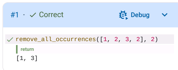
Figure 2.1. An example of how the feedback for the test suite from listing 2.1 can be rendered (in this case, it is rendered by Dodona).
