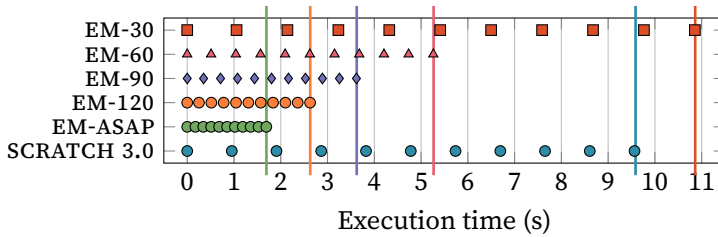
Figure 7.10. Behaviour of the Catch the apples exercise with different execution models. Marks represent score changes (or the initial score at 0), while vertical lines indicate when the player hits 10 points.
