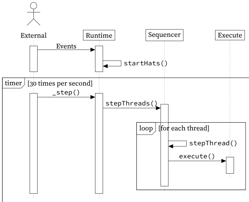
Figure 6.2. Sequence diagram showing the interactions in the virtual machine relevant to the debugger. The Runtime receives events from the user interface or from user interaction (grouped as “External” in the diagram), in response to which threads are created or removed. Meanwhile, the _step method is called 30 times per second (this is implemented inside the Runtime, but should be considered external). This method manages the threads, and calls stepThreads , which will then call stepThread for each thread in the virtual machine. This last method will finally call the execute method on the Execute class, which will do the actual executing.
